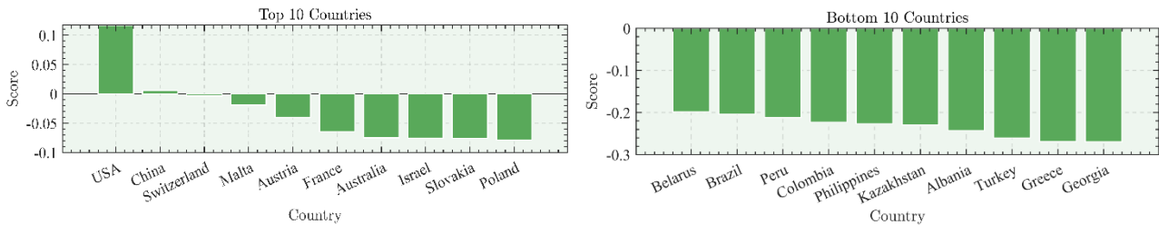
Figure 3. Score schematic
